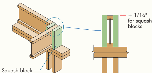
FIGURE 1 SQUASH BLOCK INSTALLATION AND CAPACITIES
